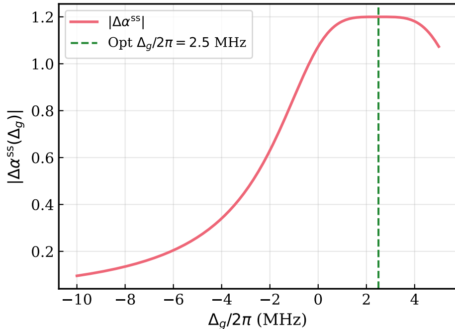
(b) Drive frequency optimization ( \chi/\kappa = 1 )
