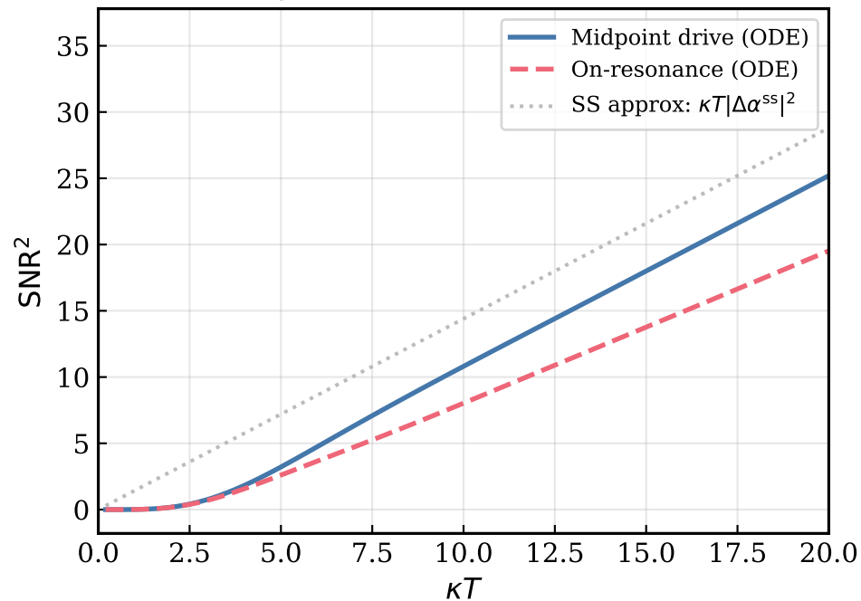
(a) Integrated \text{SNR}^2 vs readout duration
