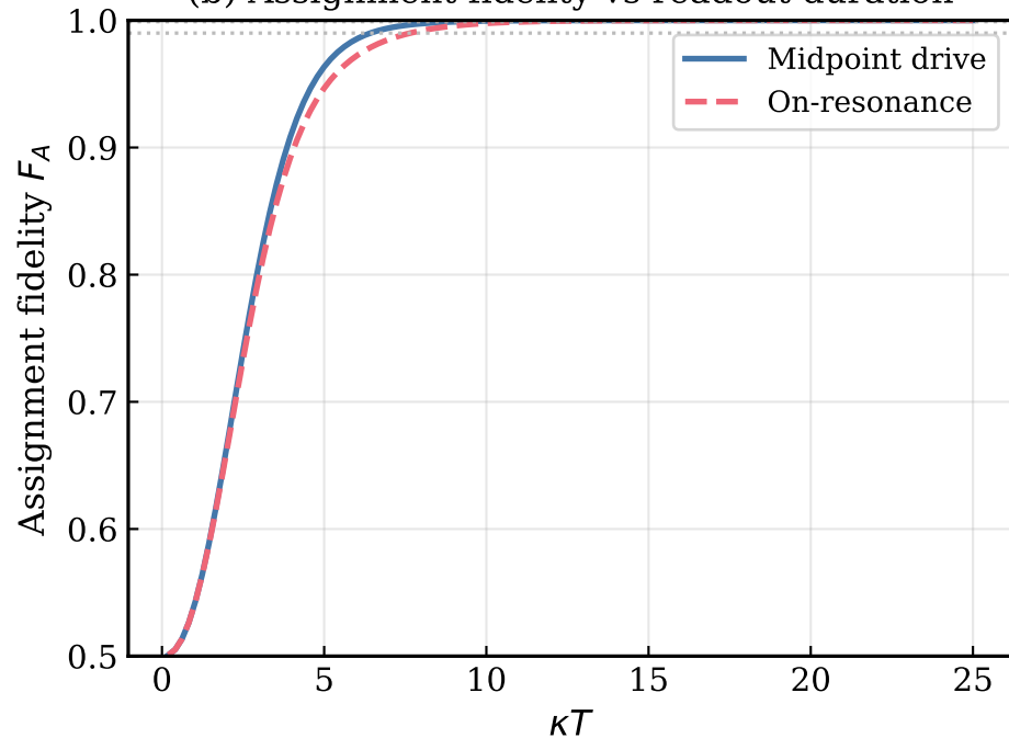
(b) Assignment fidelity vs readout duration
