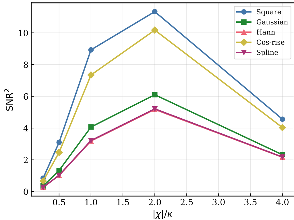
(a) \text{SNR}^2 vs \chi/\kappa ( \kappa T = 5 )
