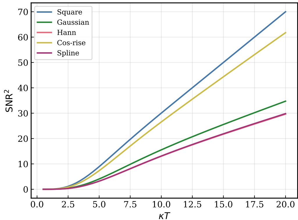
(b) \text{SNR}^2 vs \kappa T at \chi/\kappa = 1
