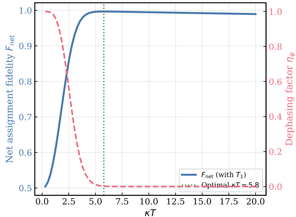
(a) Net readout fidelity vs \kappa T with T_1 and dephasing
