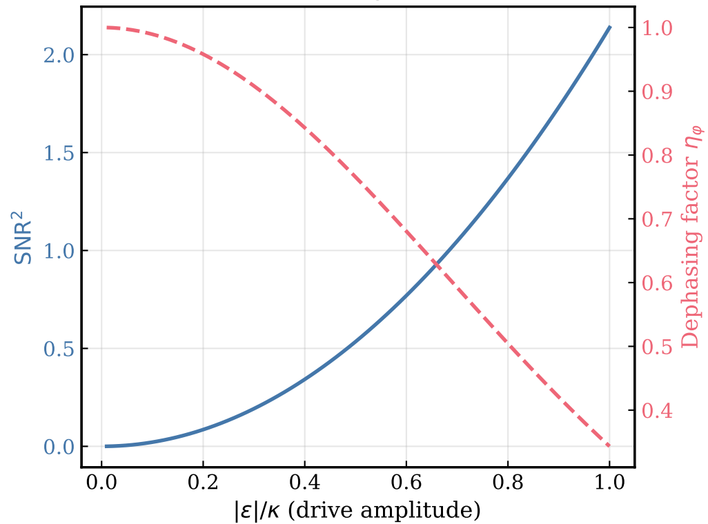
(b) \text{SNR}^2 and dephasing vs drive amplitude
