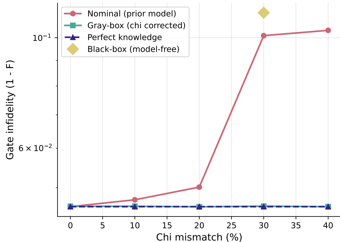
Noiseless evaluation on truth model
