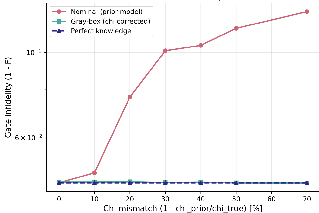
Phase 5.1: Chi mismatch sweep (noiseless)
