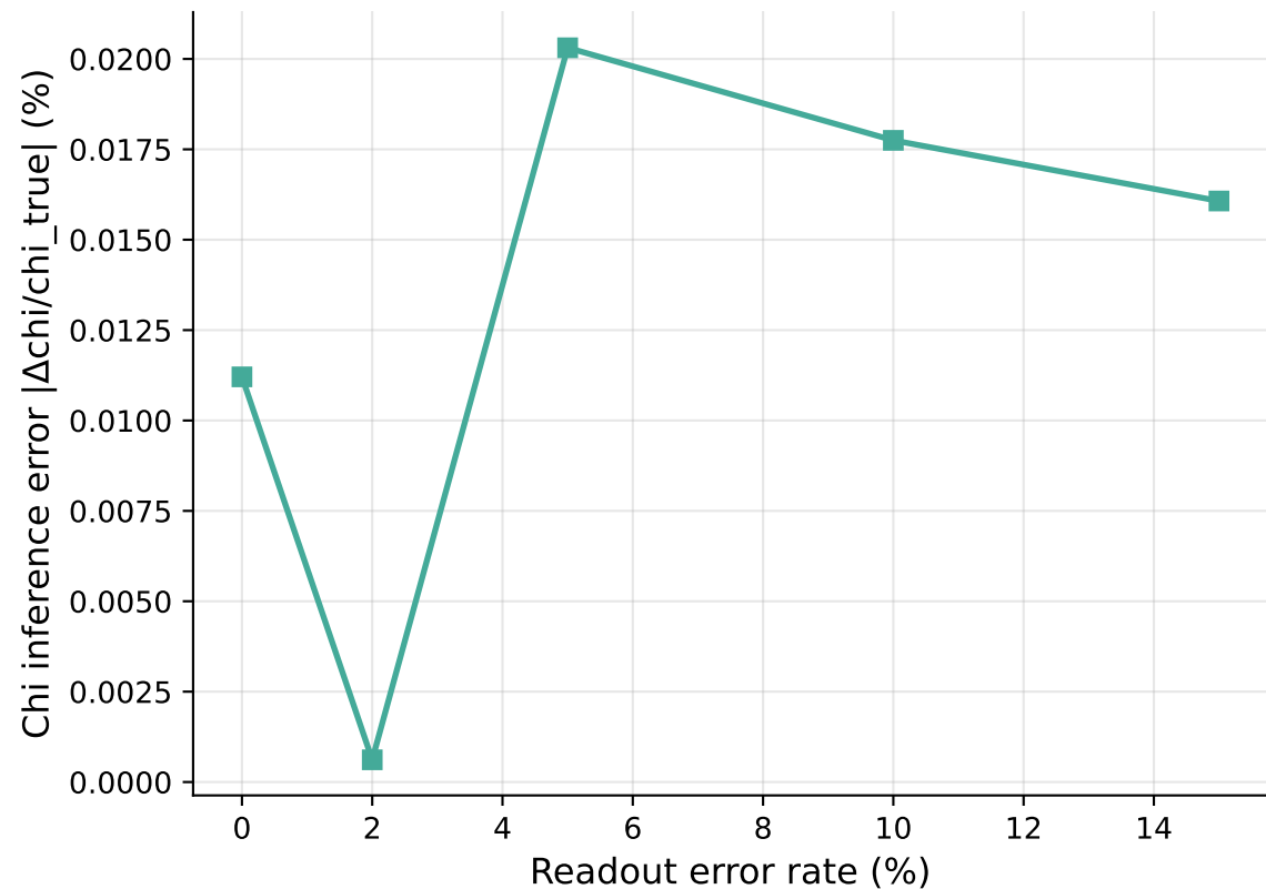
(a) Chi inference error vs readout error
