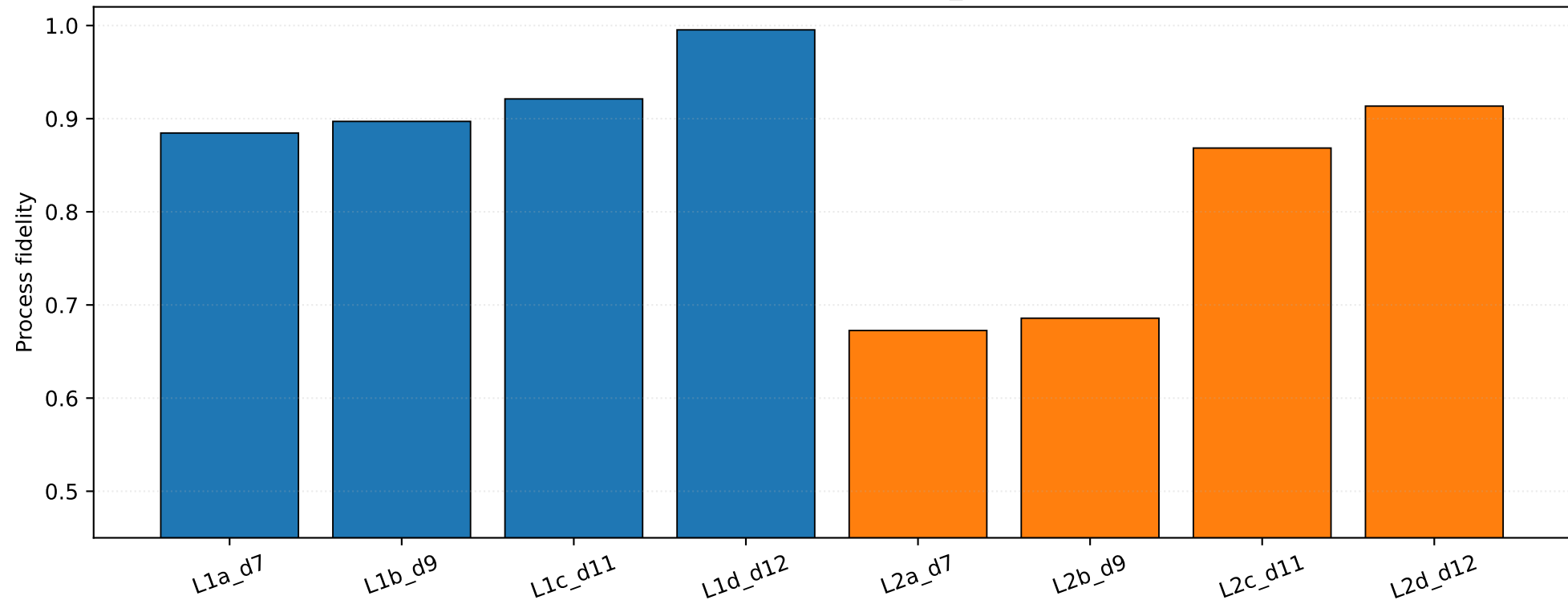
Ansatz-size scaling for structured U_{\text{target}} synthesis
