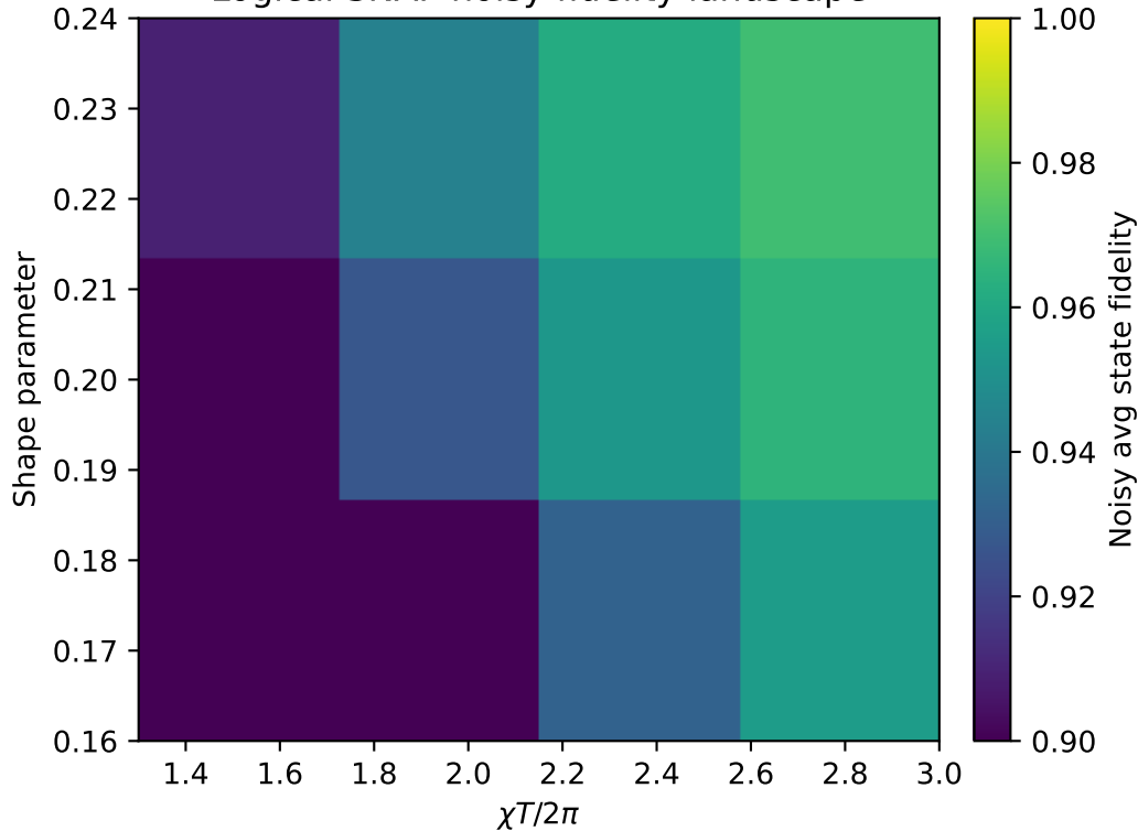
Logical SNAP noisy-fidelity landscape
