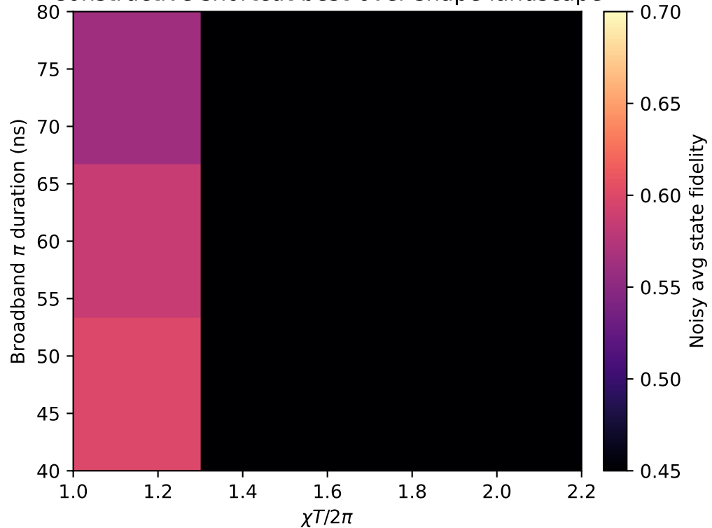
Constructive shortcut best-over-shape landscape
