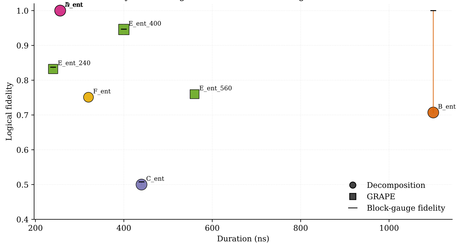
Hybrid entangler benchmark on the logical 2x2 block
