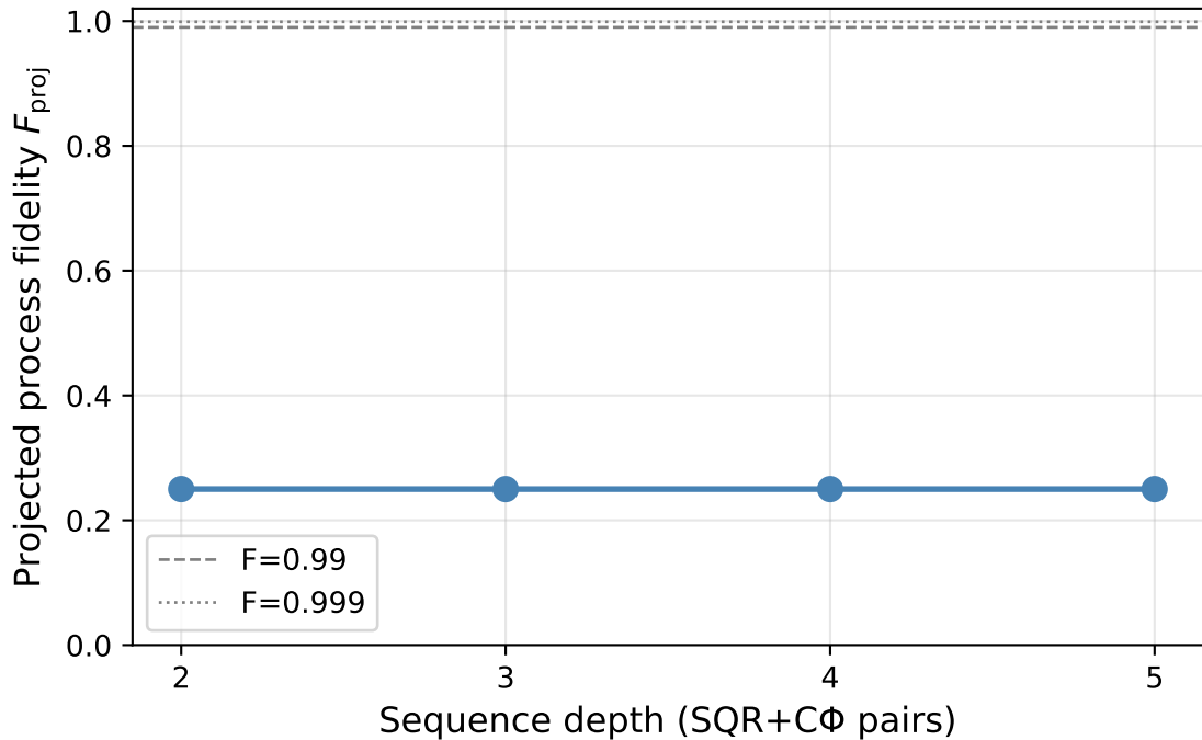
Phase 2: Depth sweep — Library B in 4D ideal space
