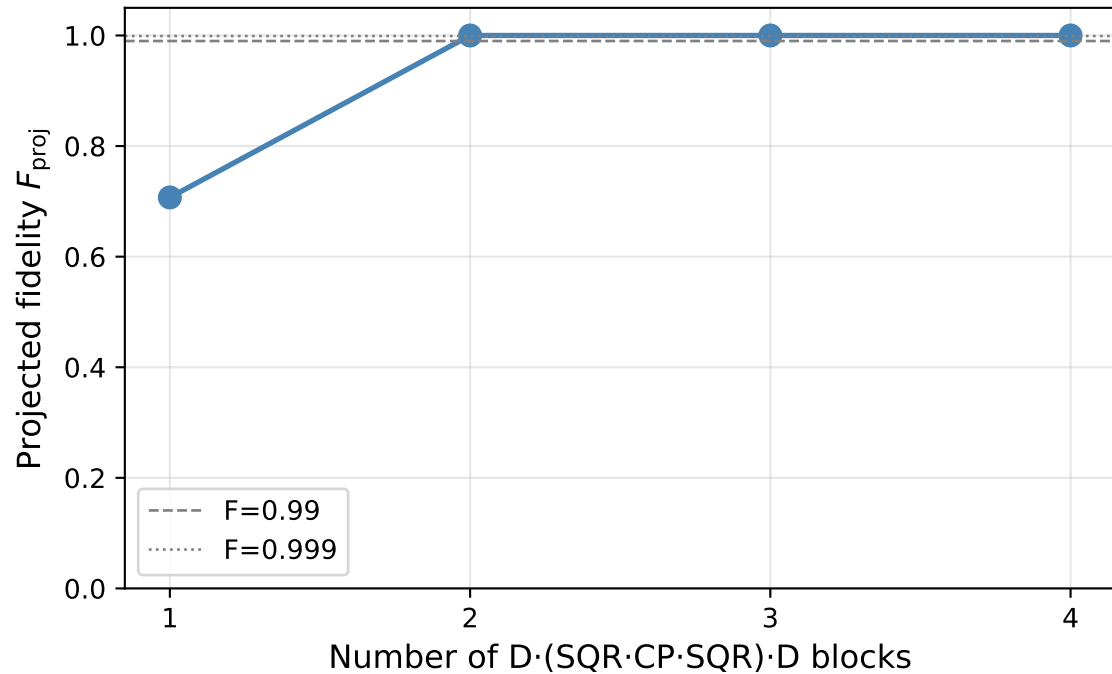
Phase 2: Depth sweep — Library B+D
