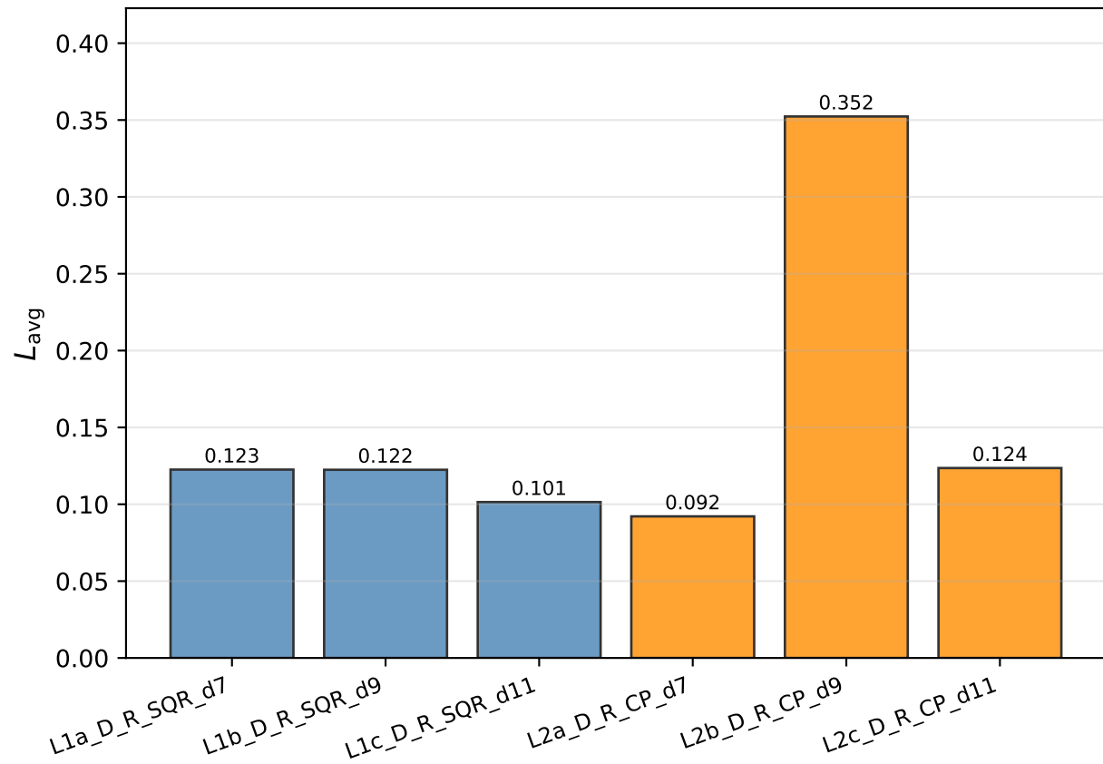
Average leakage by ansatz
