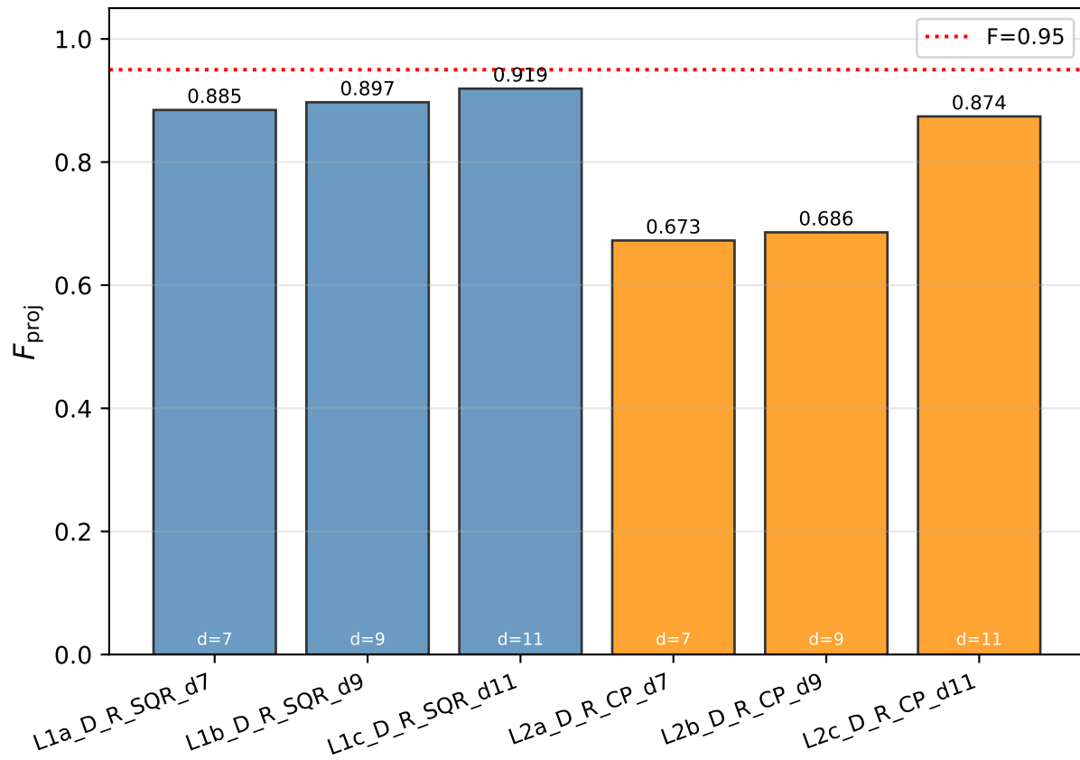
Phase 4: Subspace fidelity by ansatz (blue=Library 1 D+R+SQR, orange=Library 2 D+R+CP)
