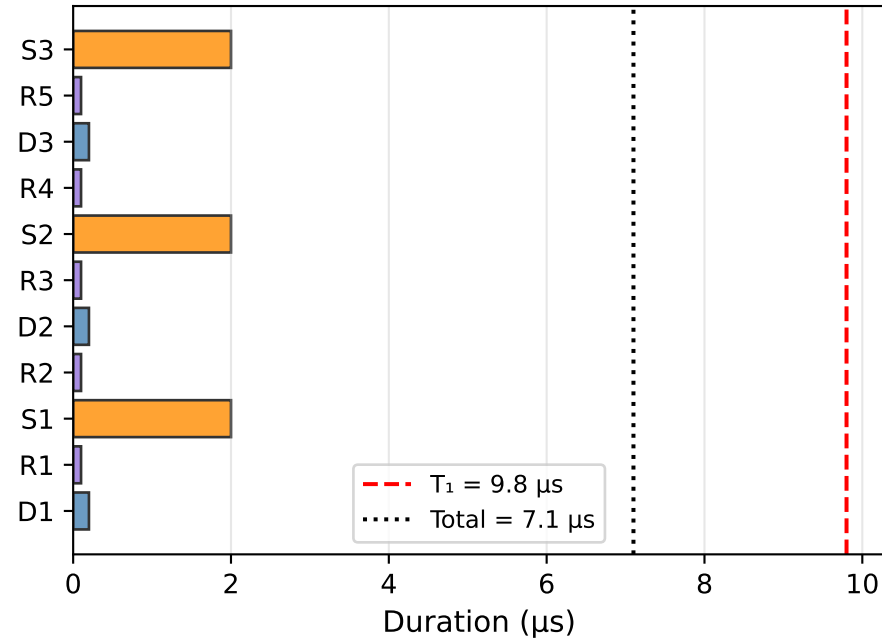
L1c gate duration breakdown
