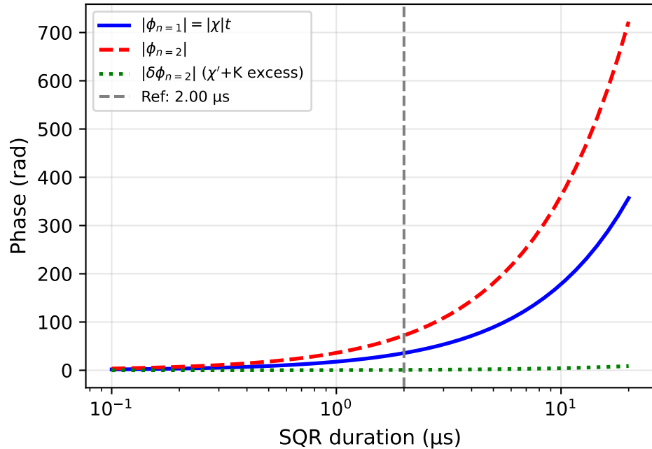
Dispersive phase during SQR pulse
