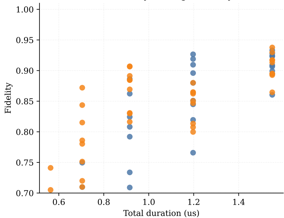
SNAP Noisy Average Fidelity
