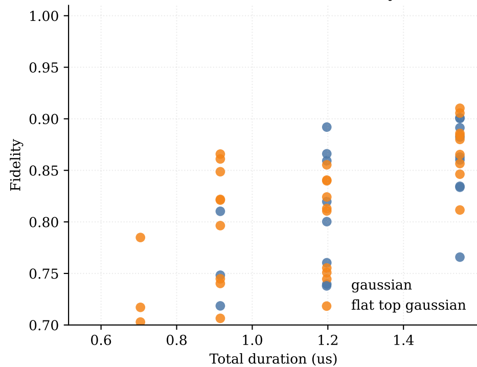
SNAP Closed Process Fidelity
