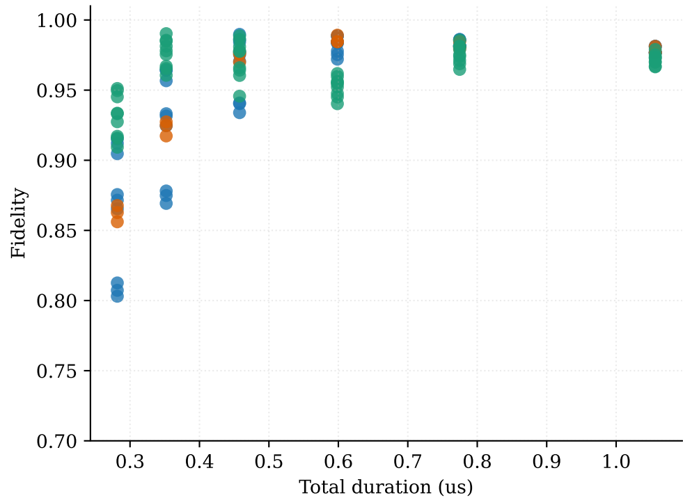
SQR Noisy Average Fidelity
