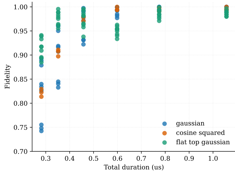
SQR Closed-System cphase Fidelity
