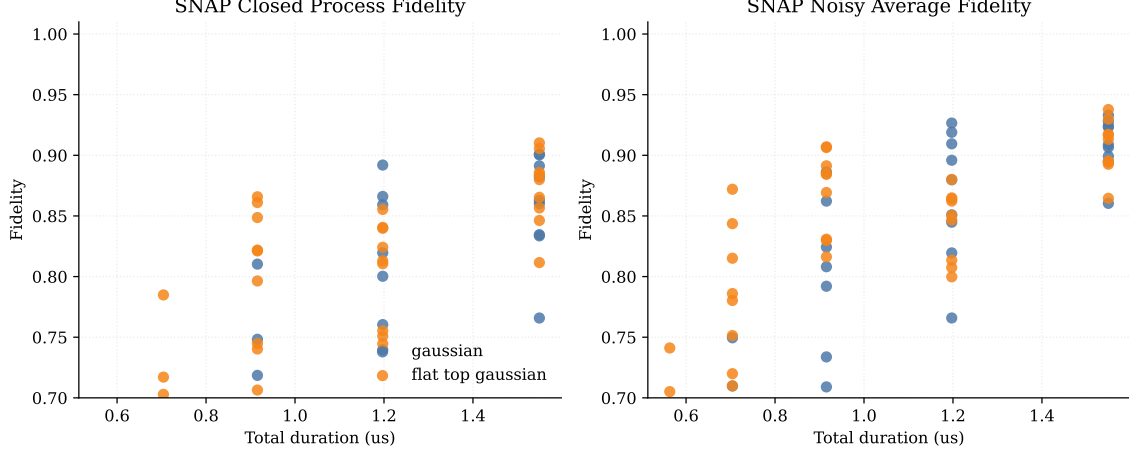
Figure 2: Closed-system and noisy SNAP performance for Gaussian and flat-top Gaussian literature-style selective pulses. The best points occur once each selective \pi pulse is long enough to resolve the number splitting but not so long that decoherence dominates.
