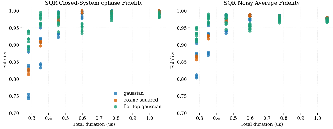
Figure 1: Closed-system and noisy SQR performance for the literature-informed pulse families. Gaussian and cosine-squared pulses dominate the long-duration closed-system regime, while the best noisy operating point shifts to a shorter flat-top Gaussian pulse. Horizontal structure in the noisy panel reflects the fact that several shape and amplitude variants cluster near the same practical fidelity.
