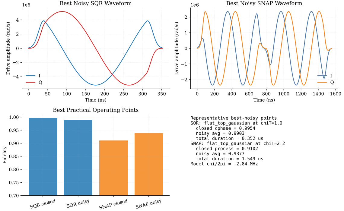
Figure 3: Optimized noisy-reference waveforms and summary fidelities. The best noisy SQR point is a short flat-top Gaussian pulse at |\chi|T/2\pi = 1 , while the best SNAP point is a two-pulse flat-top Gaussian sequence at |\chi|T_\pi/2\pi = 2.2 .
