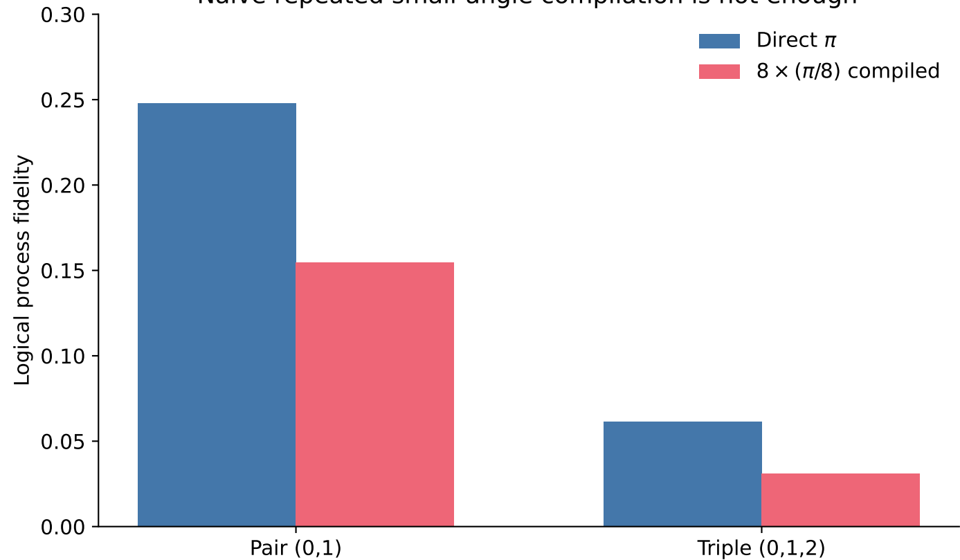
Naive repeated small-angle compilation is not enough
