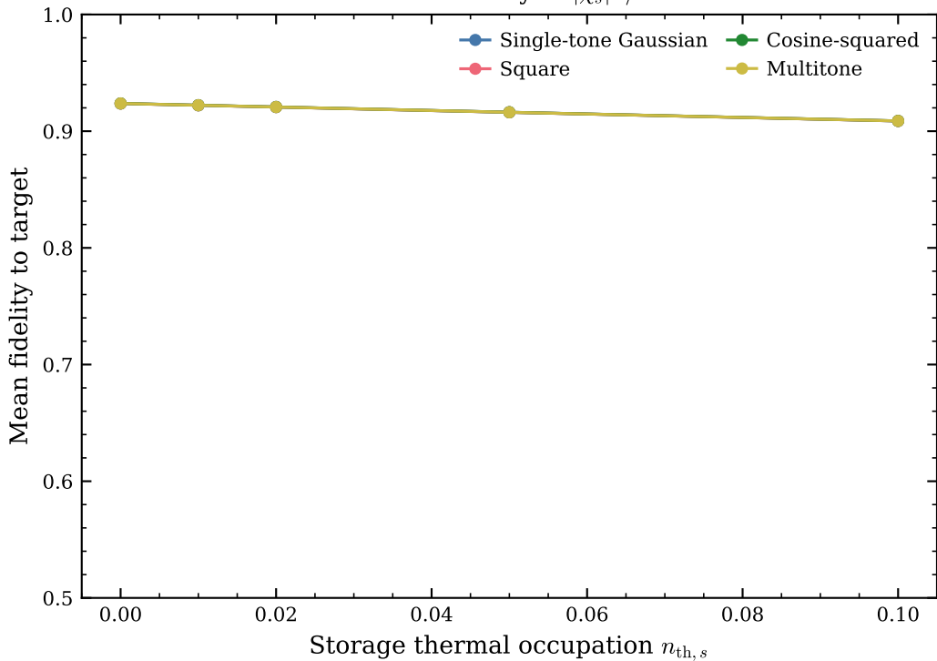
Thermal sensitivity at |\chi_s|T/2\pi = 2.0
