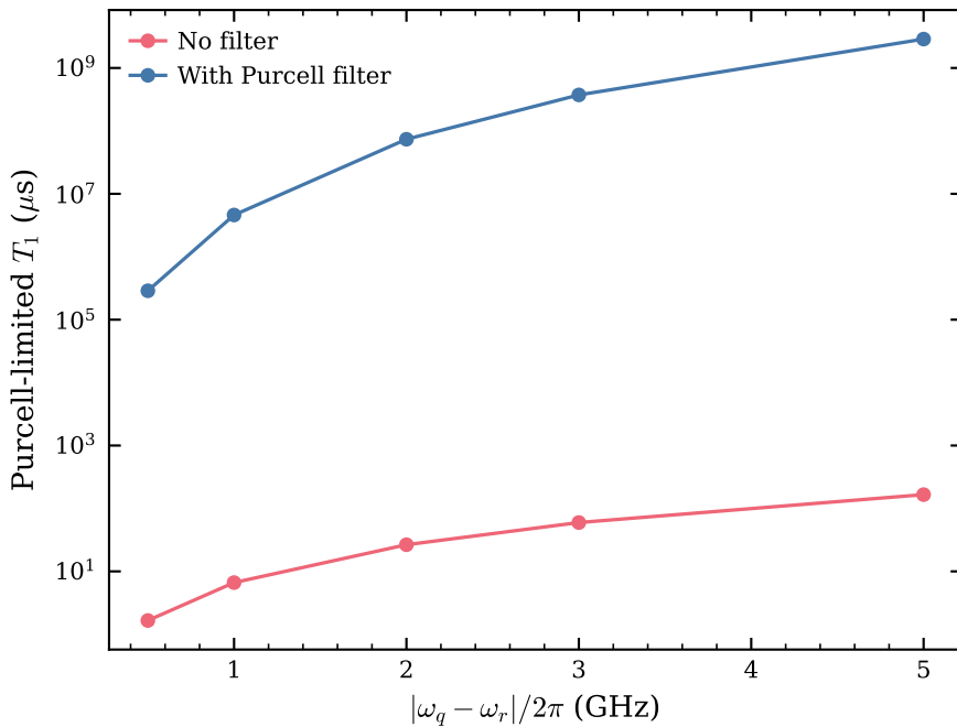
Purcell protection from the readout chain
