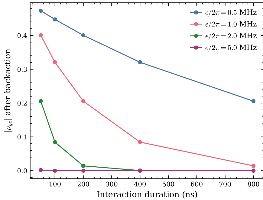
Measurement-induced dephasing
