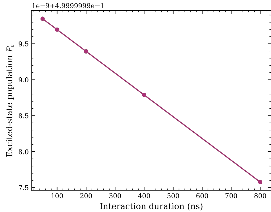
Readout-induced relaxation
