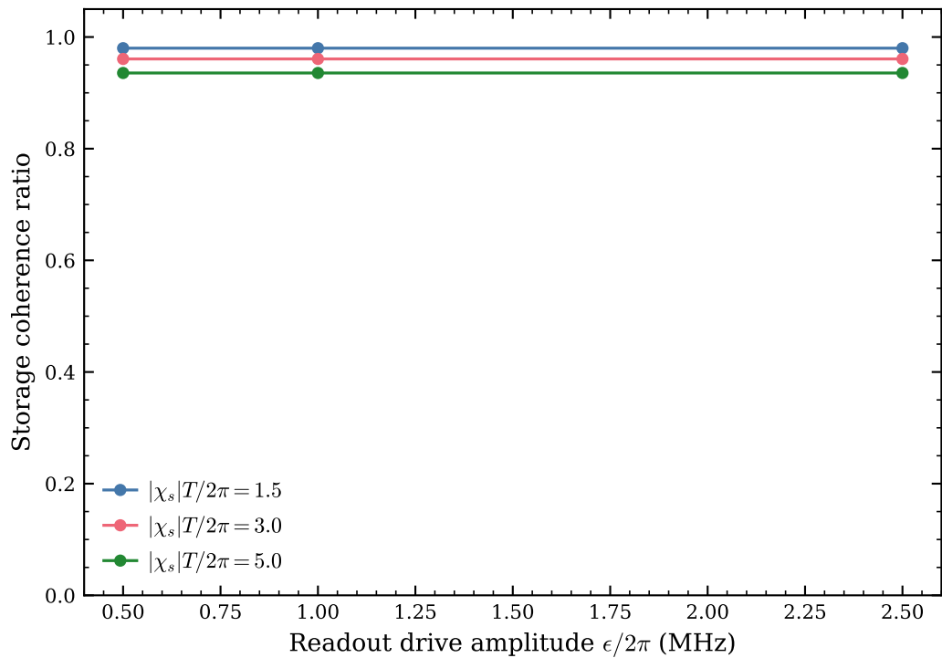
Readout-induced storage dephasing for Square
