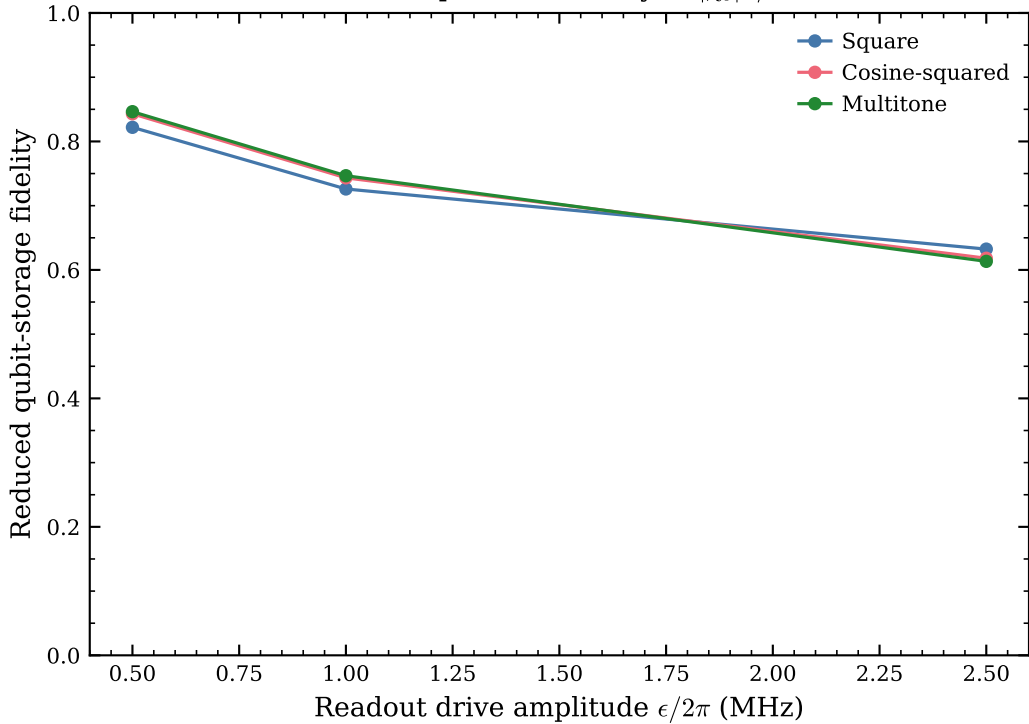
Three-mode spectator fidelity at |\chi_s|T/2\pi = 3.0
