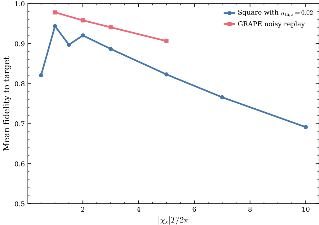
Parametric baseline versus GRAPE under realistic noise
