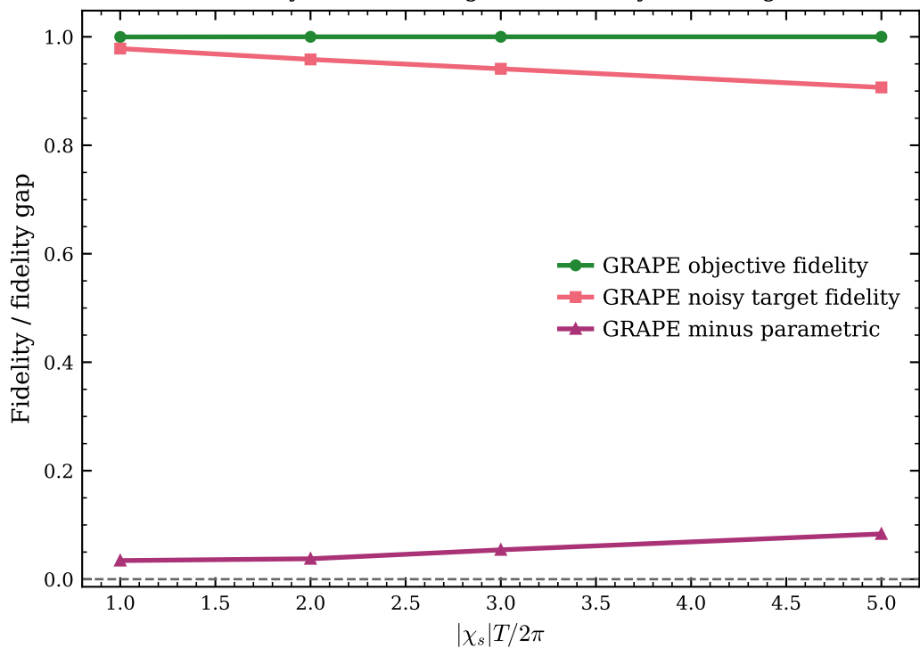
Closed-system advantage versus noisy realized gain
