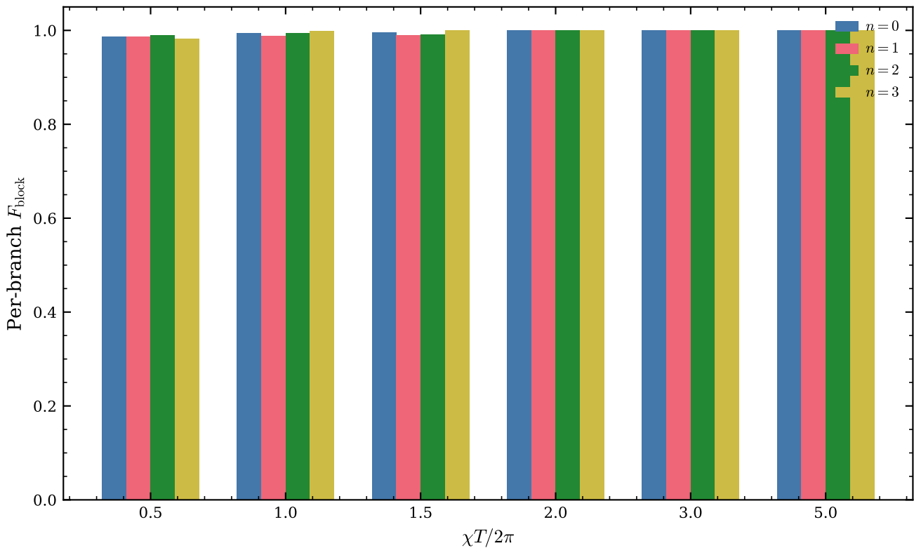
DE+NM per-branch fidelity (all-branch target)
