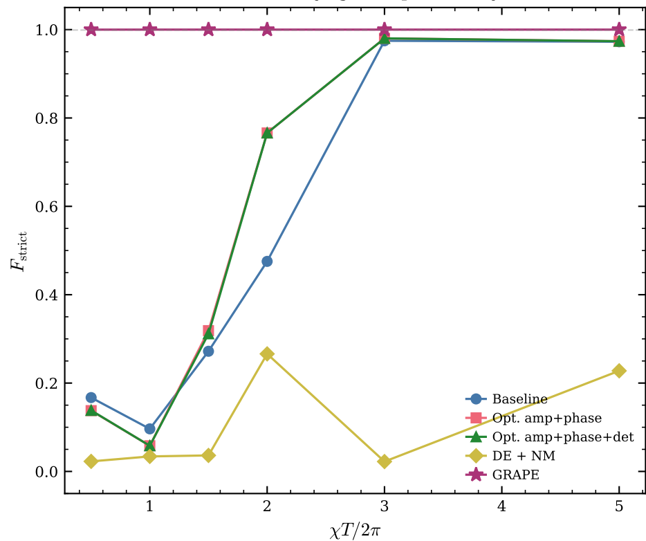
Strict fidelity (global phase only)
