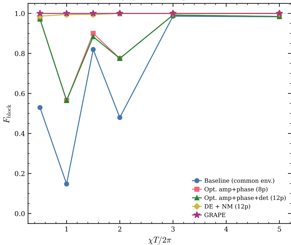
Block fidelity (per-branch phase freedom)
