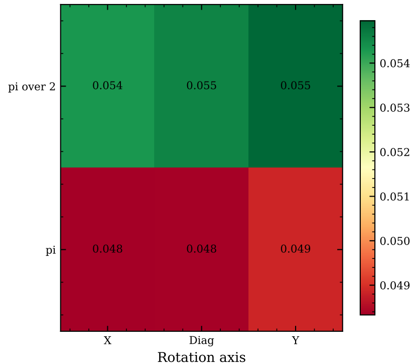
Echoed single-tone logical fidelity\n(at \chi T/2\pi = 3 )
