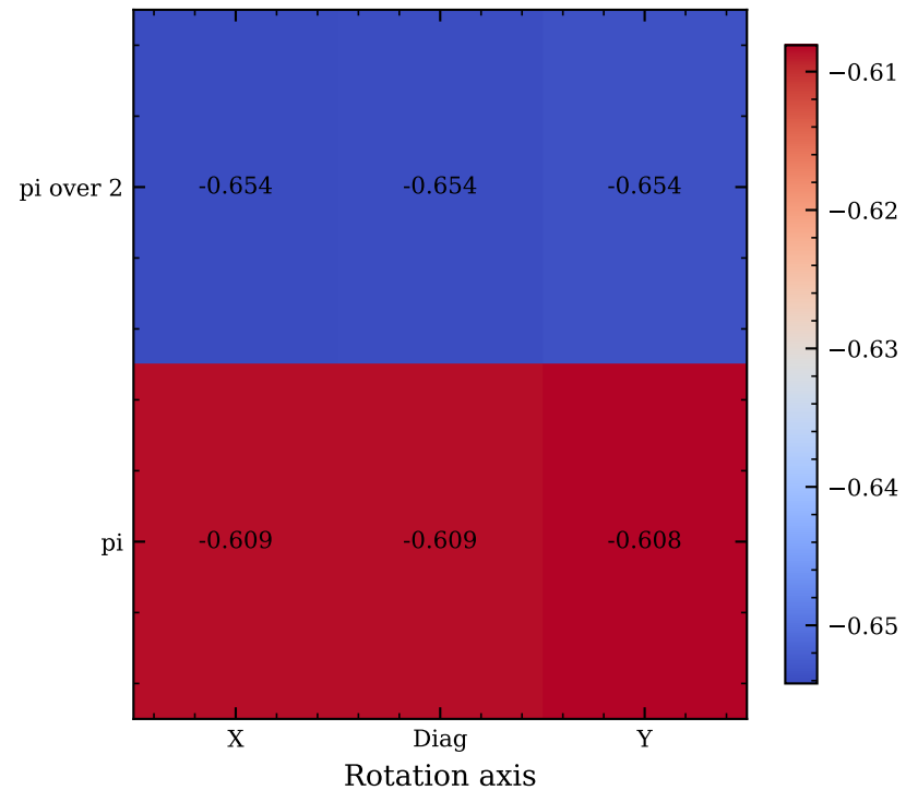
Echo gain in logical fidelity\n(at \chi T/2\pi = 3 )
