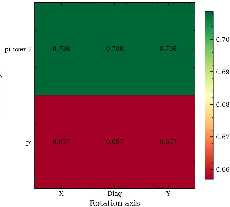
Single-tone logical fidelity\n(at \chi T/2\pi = 3 )
