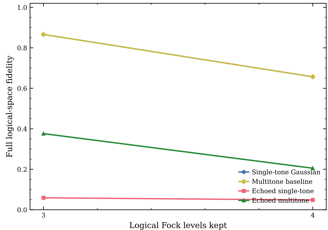
Logical fidelity vs truncated logical subspace ( \theta = \pi , X-axis, n_0 = 1 , \chi T/2\pi = 3 )
