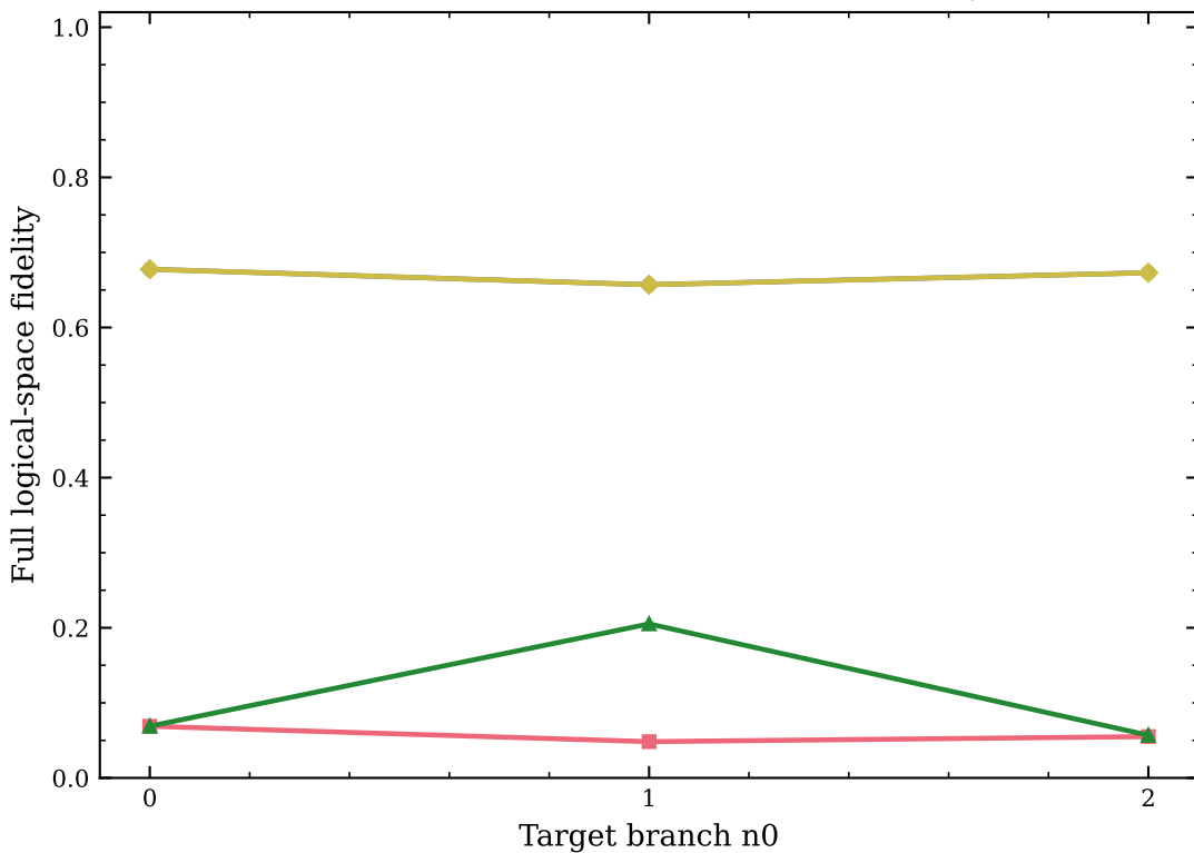
Logical fidelity vs target branch ( \theta = \pi , X-axis, \chi T/2\pi = 3 )
