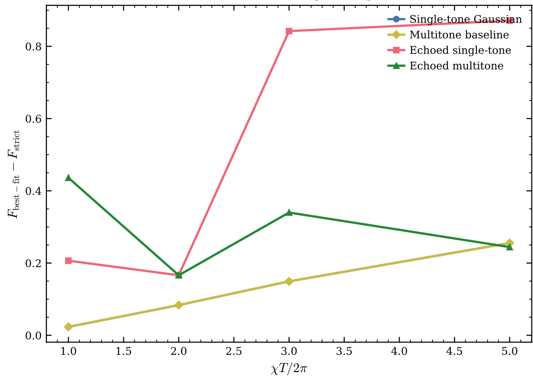
Gain from fitted cavity block phase
