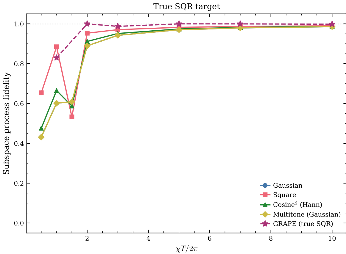
SQR fidelity vs \chi T/2\pi (target branch n_0 = 1, \theta = \pi )
