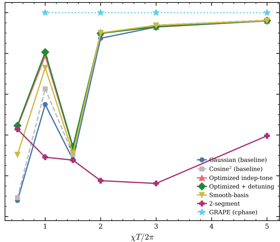
Block-phase-relaxed fidelity \mathcal{F}_{\text{block}}
