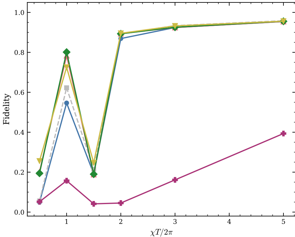
Strict logical fidelity \mathcal{F}_{\text{strict}}
