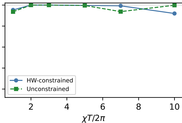
True SQR (GRAPE)
