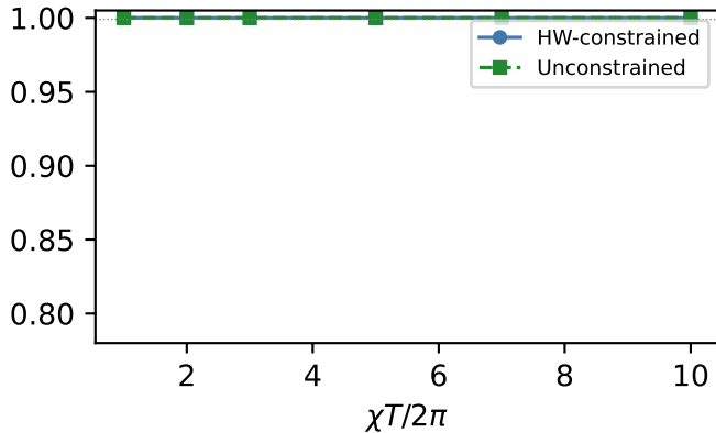
Cphase SQR (GRAPE)
