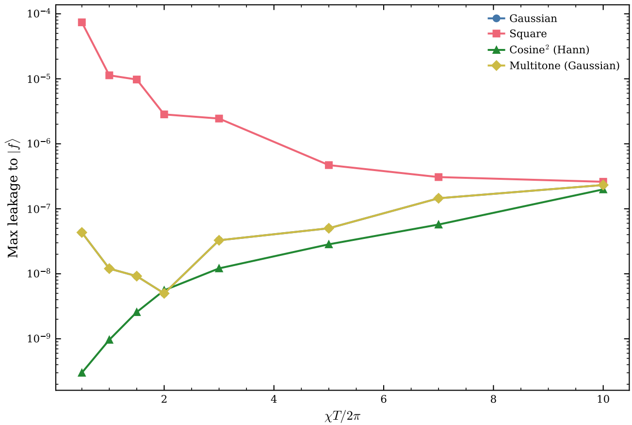
Leakage to third transmon level ( n_{\text{tr}} = 3 )
