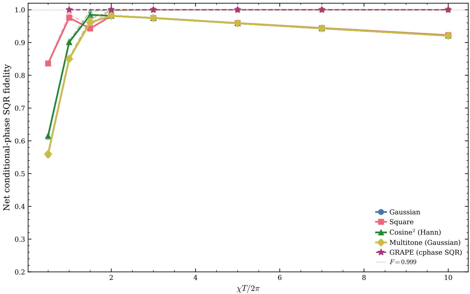
Net fidelity including \chi' , K , T_1 , T_2 (dashed: ideal closed-system; solid: full model)
