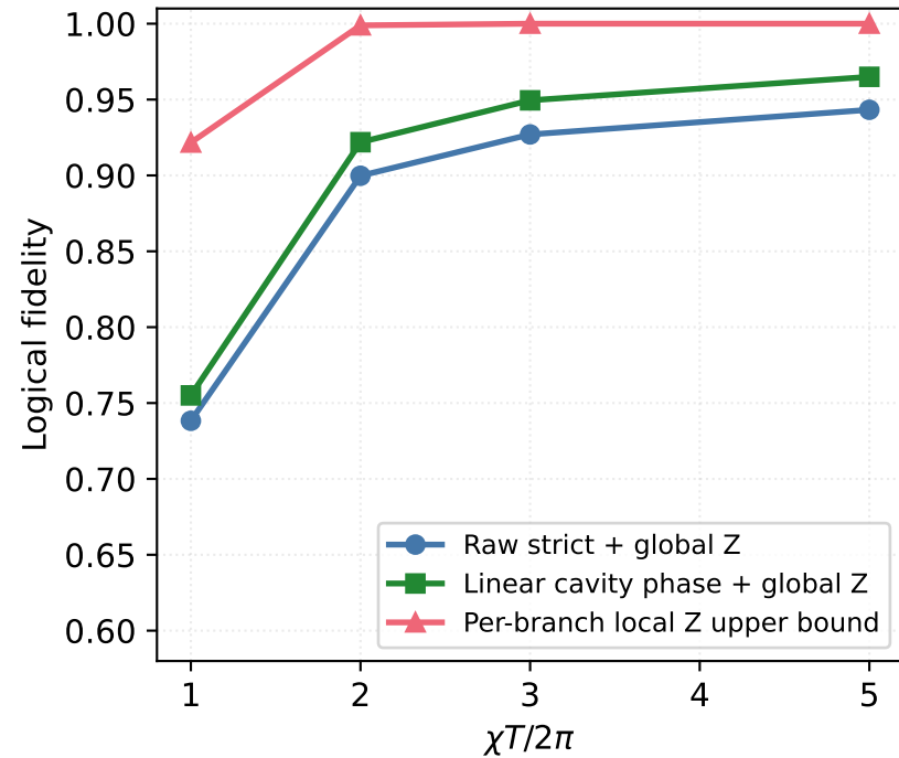
Gaussian
