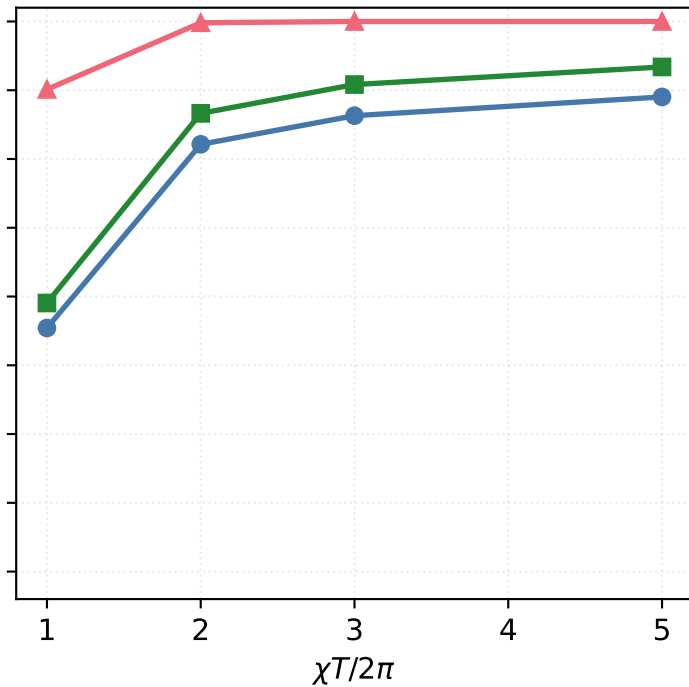
Cosine-squared
