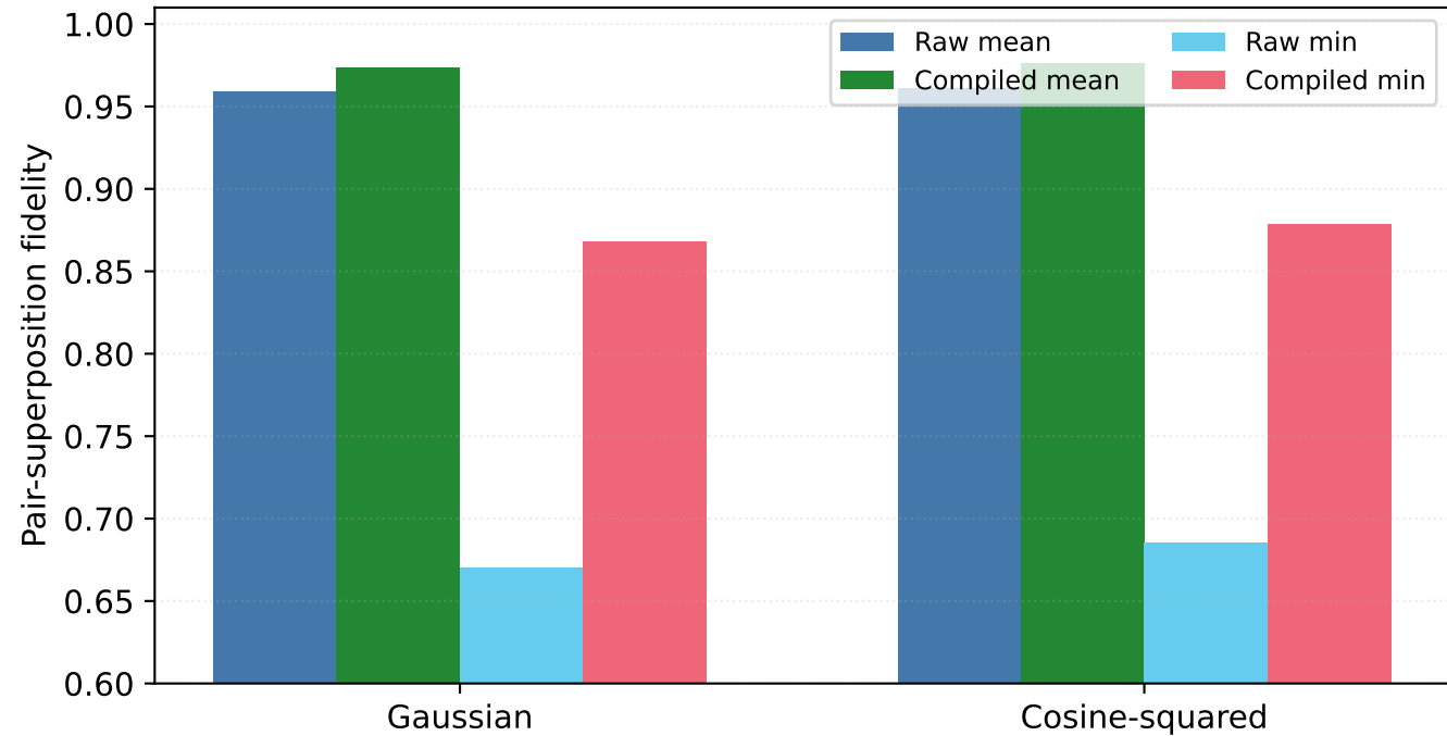
Coherence benchmark over |g, n\rangle \pm |g, m\rangle , |e, n\rangle \pm |e, m\rangle , and |g, n\rangle \pm |e, m\rangle probes
