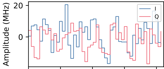
HW-constrained GRAPE pulse ( \chi T/2\pi = 3 )
