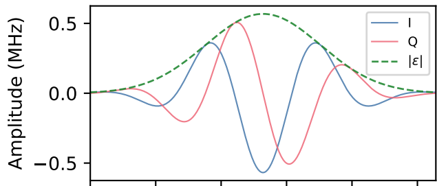
Cosine-squared
