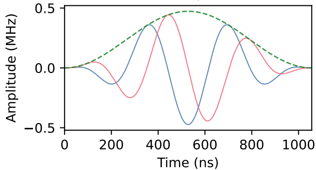
Cosine-squared
