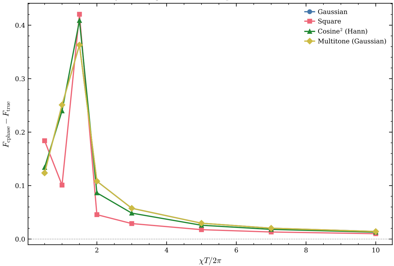
Fidelity advantage of conditional-phase SQR over true SQR
