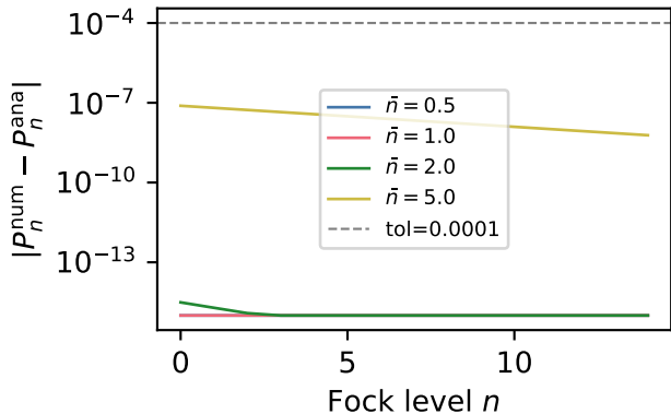
P_n deviation from analytic
