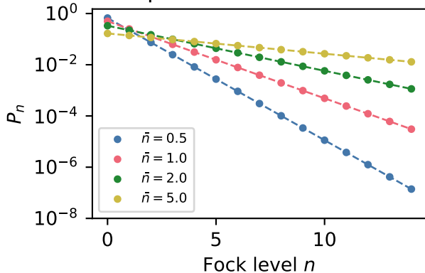
Thermal photon-number distributions
