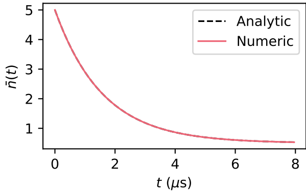
Cooling: n_0 = 5.0, n_{th} = 0.5
