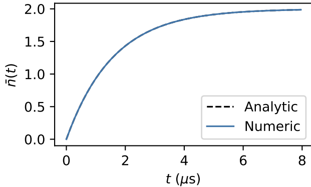
Heating: n_0 = 0, n_{th} = 2.0
