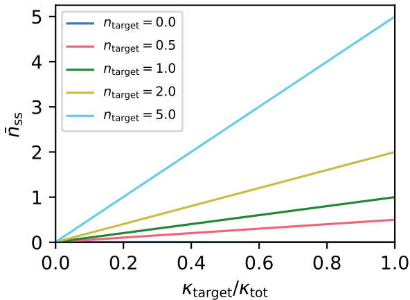
\bar{n}_{ss} vs coupling fraction
