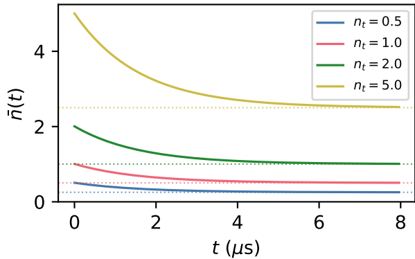
Cooling: \bar{n}(0) = 2\bar{n}_{ss}
