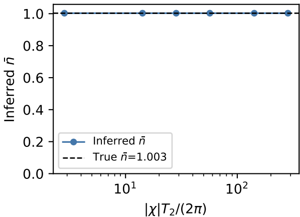
Ramsey inference bias vs qubit T_2
