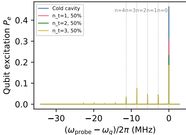
Number-selective spectroscopy
