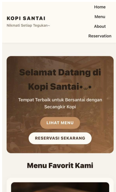
HomePage (Mobile)
