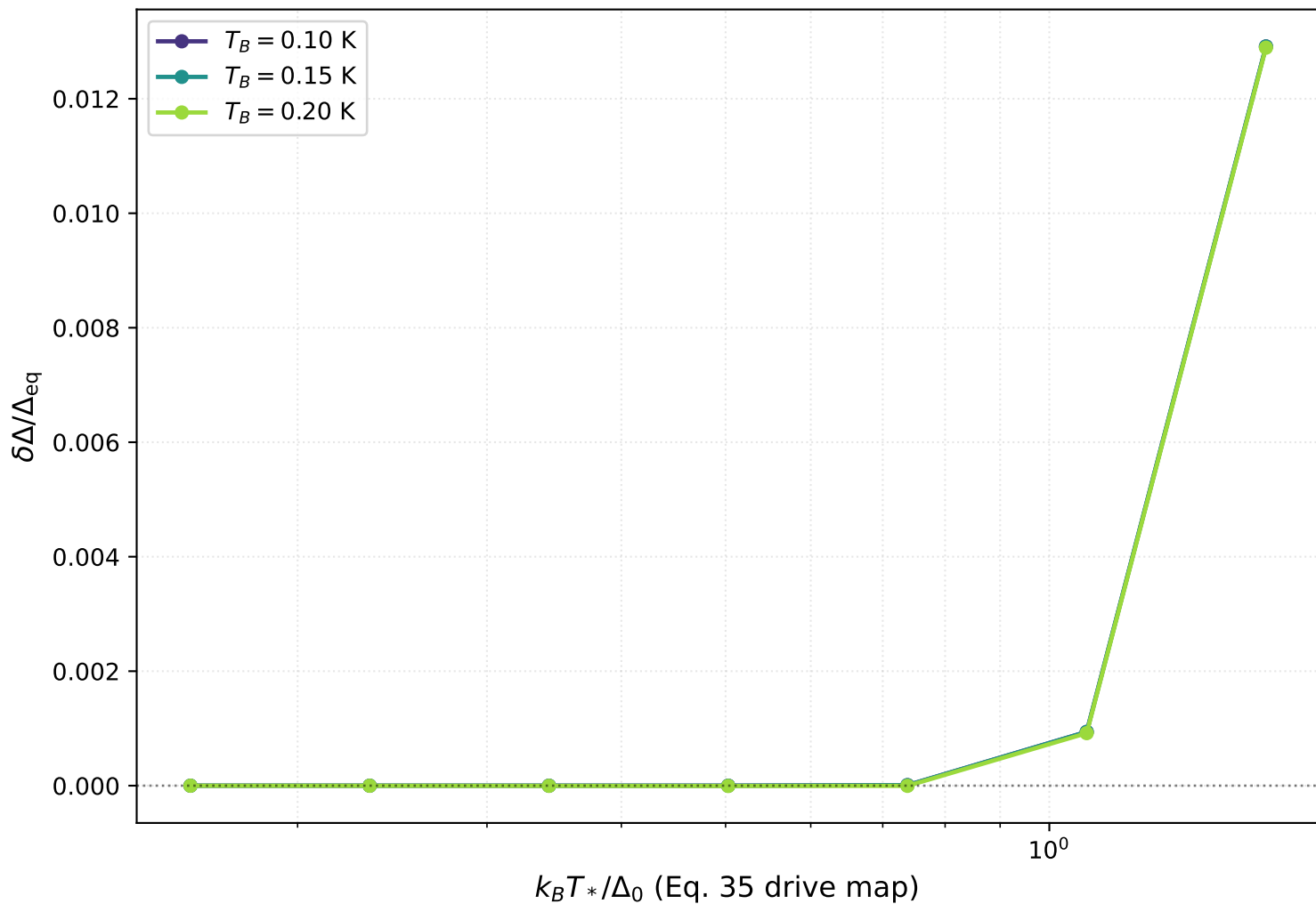
Fischer 2023 Fig. 6 characterization Ph0-Kaplan (acoustic-escape \tau_l ) + self-consistent gap
