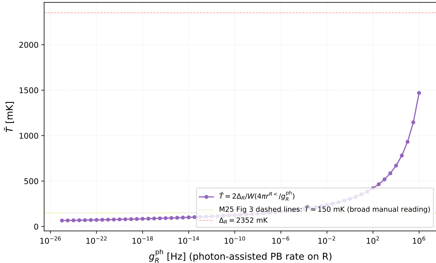
M25 Eq. 8 transcription: Lambert-W self-regression (one manual broad paper anchor; no digitized paper points) Fig 3 params: \Delta_R/h = 49 GHz, r^R < = 6.25 MHz
