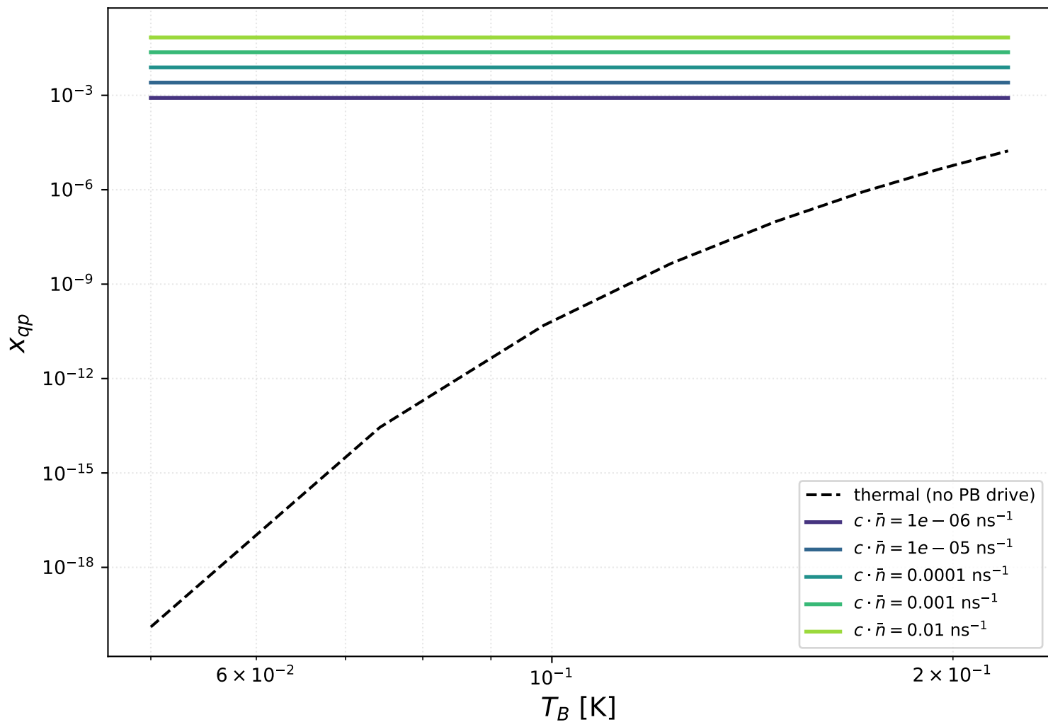
Fischer & Catelani 2024 Fig 8 — PB-photon drive
