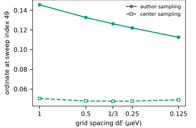
FIG. 2. Grid refinement of the anchored-point ordinate ( T_B = 0.20 \text{ K} , sweep index 49) under both readings of the re-solved root. The center-carrier reading is grid-converged at the published resolution; the left-edge reading is not.
