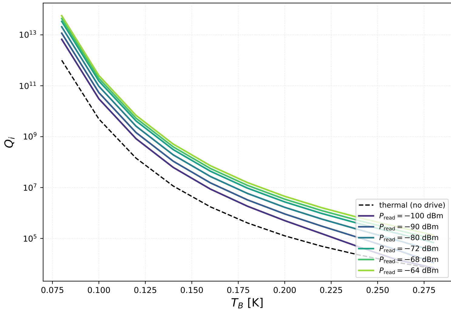
Fischer 2023 Fig 7 — Q_i(T_B) with \bar{n} loop \Delta_0 = 180 \text{ } \mu\text{eV} , \omega_0 = \Delta_0/9 , \alpha = 0.5 , Q_c = 100000
