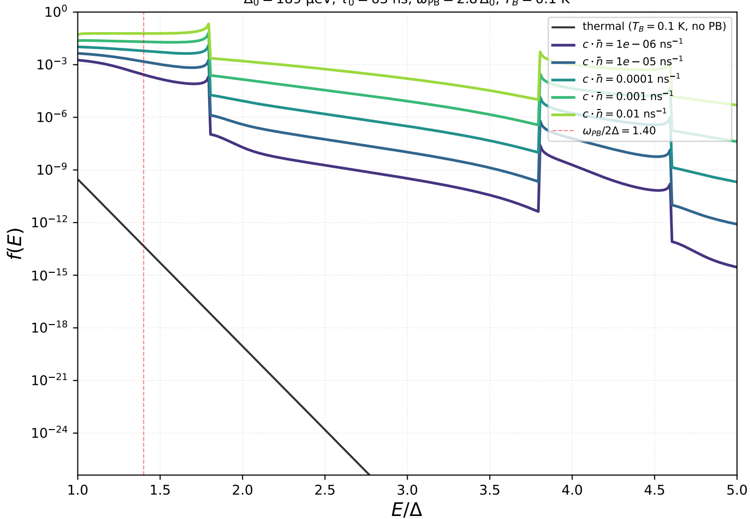
Fischer & Catelani 2024 Figs 5-7 — PB-photon drive at fixed T_B
